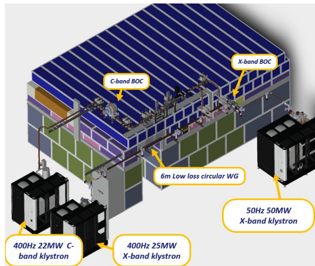
Figure 1: Configuration of the TEX facility area around the bunker, after the upgrade, with the three RF power sources.
