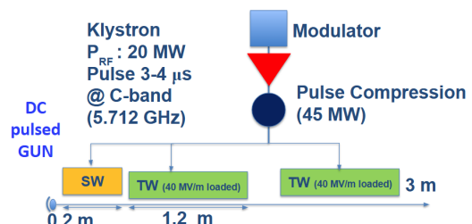
Figure 1: Accelerator layout scheme.
