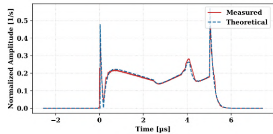
Figure 5: Low power test measurements vs. theoretical results.
