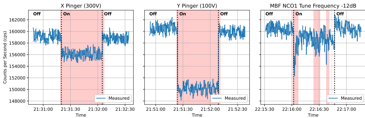
Figure 3: Examples of raw data from the Collimator BLD showing the effects on the loss rate of turning on and off various disturbances. The shaded red sections show where the anomaly detection indicates an anomaly for a correctly predicting model.
