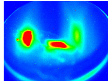
Figure 3: Injected and first turn beam seen on the screen monitor located downstream of the thin septum.
