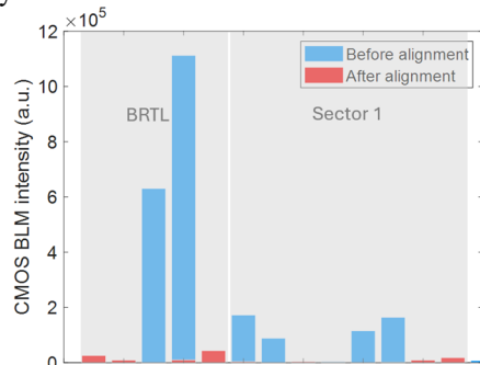
Figure 1: Change in the loss pattern in the BRTL, injection straight and Arc 01 as detected by the CMOS BLMs before (blue) and after the (orange) vacuum valve realignment.
