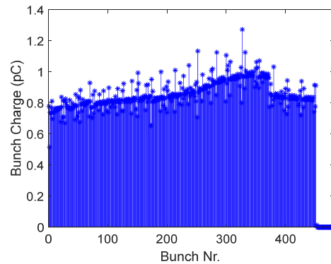
Figure 6: Fill pattern during nominal operation at 400 mA with a 30-bucket gap. The charge per bunch is calculated from PCT current readings. The filling pattern feedback loop was not closed when this data was acquired.
