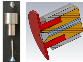
Figure 3: Third generation home made pick-ups.
