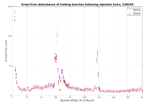
Figure 6: IK disturbance to the trailing bunches.
