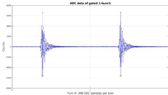
Figure 4: ADC waveform data of one selected bunch as detected by a Spark unit. Two-turn signals are plotted for one bucket; 398 ADC samples per turn.
