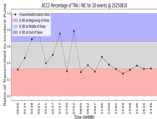
Figure 6: Location of reflection in pulse for ACC2 events.
