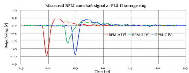
Figure 5: A measured raw BPM signal with test BPM at the PLS-II storage ring.
