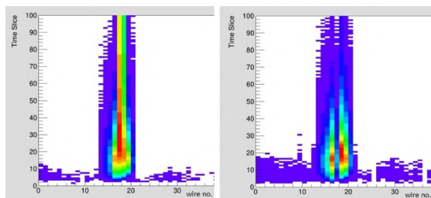
Figure 6: Development of the beam profile during a 70 \mu s macro pulse before (left) and after (right) destruction of one wire. A time slice corresponds to 5 \mu s.
