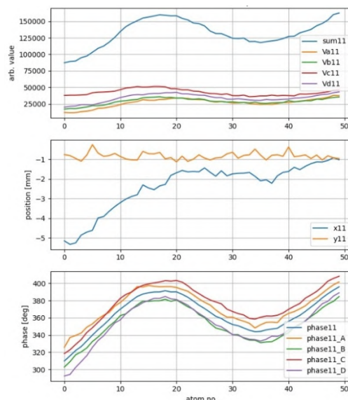
Figure 7: Position and phase measurement from LSPH. Upper: button signals and sum signal over 50 \mu s. Middle: position values. Lower: corresponding phase.
