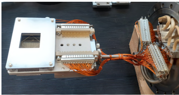
Figure 3: SEM harp by PROACTIVE. The grid consists of two harps rotated by 90°, area 32 mm x 32 mm with diamond shaped cleaning electrode, 64 wires per harp, wire pitch 0.5 mm, thickness 100 \mu\text{m} .
