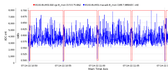
Figure 3: The gain of the BLD was switched from 0.7 V to 0.5 V at injection to avoid ADC saturation.
