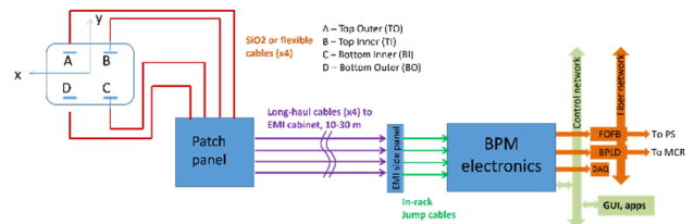
Figure 1: Block diagram of BPM wire connections.
