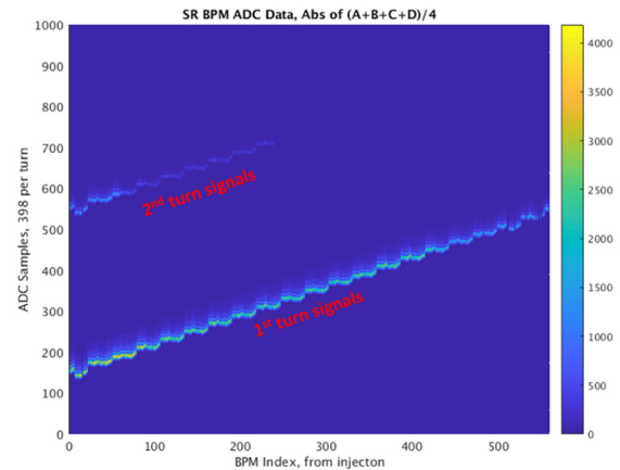
Figure 3: Raw ADC data of the first turn beam circulating in the ring.
