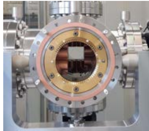
Figure 5: Look into the scraper in the beam plane. The 4 jaws from top, bottom, and the sides are partially moved in [10].
