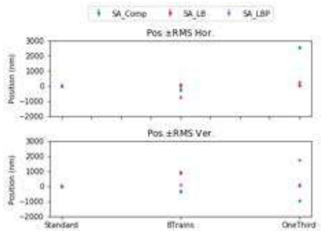
Figure 8: Positions for different FP measured with different electronics: PT-Libera Spark (blue), Libera Brilliance (red), Libera Brilliance+ (violet).
