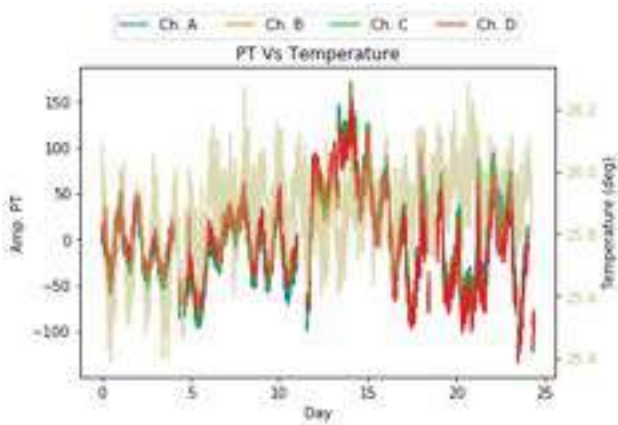
Figure 4: PT compensation data for each BPM button and temperature in the rack.
