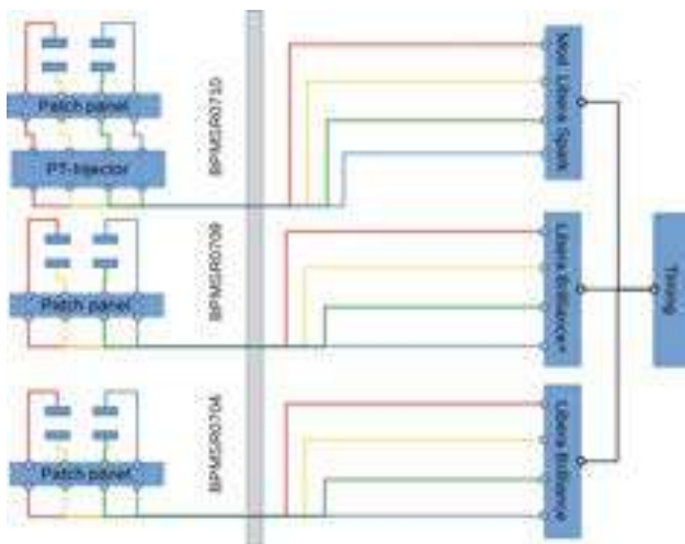
Figure 2: Schematic of the different readout system distribution.
