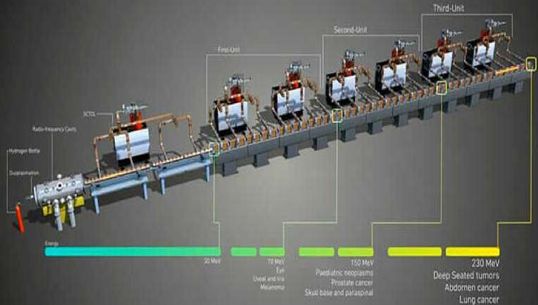
Applications of Accelerators and Detectors to Medicine [ ADAM ] A proton therapy center based on LIGHT
