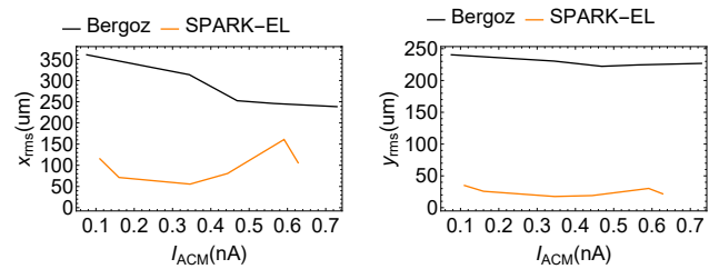
Figure 6: Comparison between the SPARK-EL and the Bergoz at BTS BPM 5.
