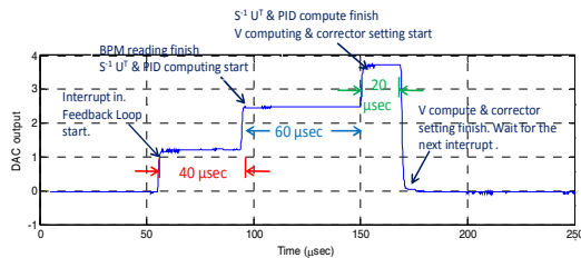
Figure 4: DAC output level is changed when each computing step is finished. The interval between two adjacent difference levels represents the respective latency for each computation.
