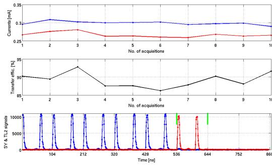
Figure 5: Injection of two bunches
