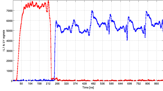
Figure 2: Injection of long bunch at 1.1 mA. The excessive length of the pulse form TL1 can be observed.
