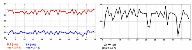
Figure 8: RMS values of the injection efficiency measurement
