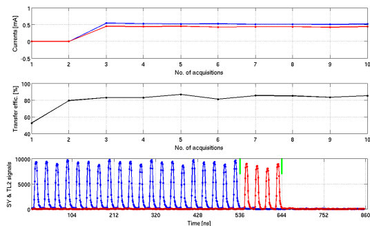
Figure 6: Injection of four bunches
