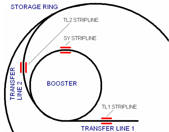
Figure 1: Injection system at ESRF lightsource
