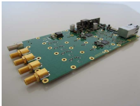
Figure 3: Prototype board.
