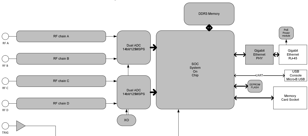
Figure 1: Basic HW design
