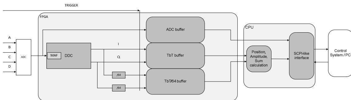
Figure 2: Functionality in the SoC
