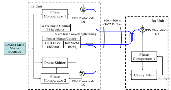
Figure 1: Simple block diagram of the Libera Sync for 500 MHz operation.
