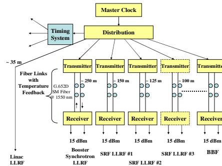
Figure 3: RF reference distribution scheme for the TPS.
