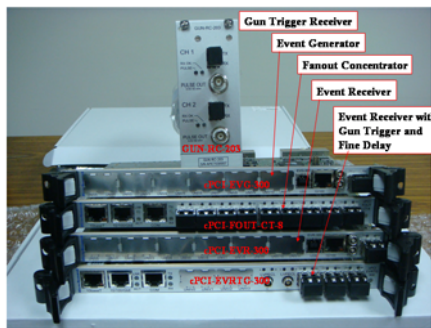
Figure 5: TPS timing modules.
