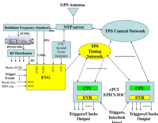
Figure 4: Block diagram of the TPS event system.
